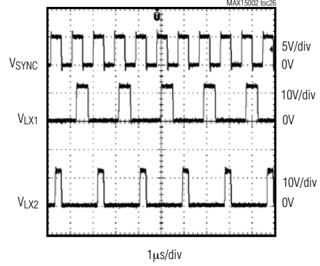
180° OUT-OF-PHASE OPERATION
